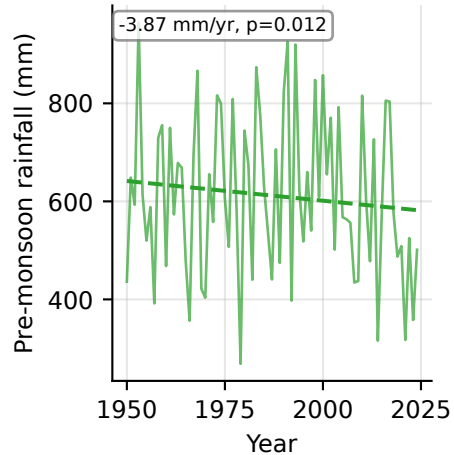
ERA5-Land trans-boundary 1950-2024
