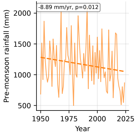
ERA5-Land Sylhet 1950-2024
