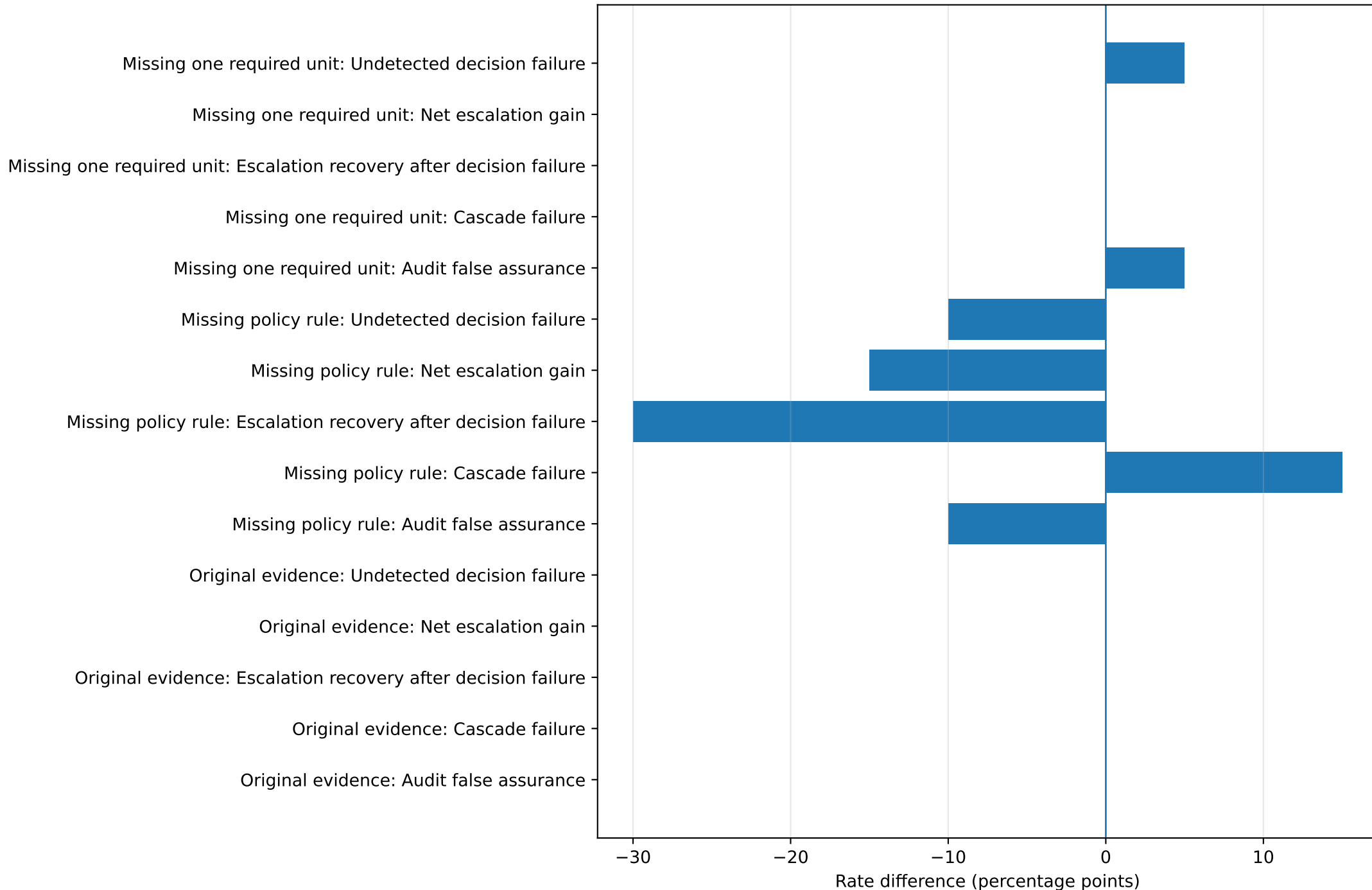
Reliability cascade metric differences: Claude minus GLM
