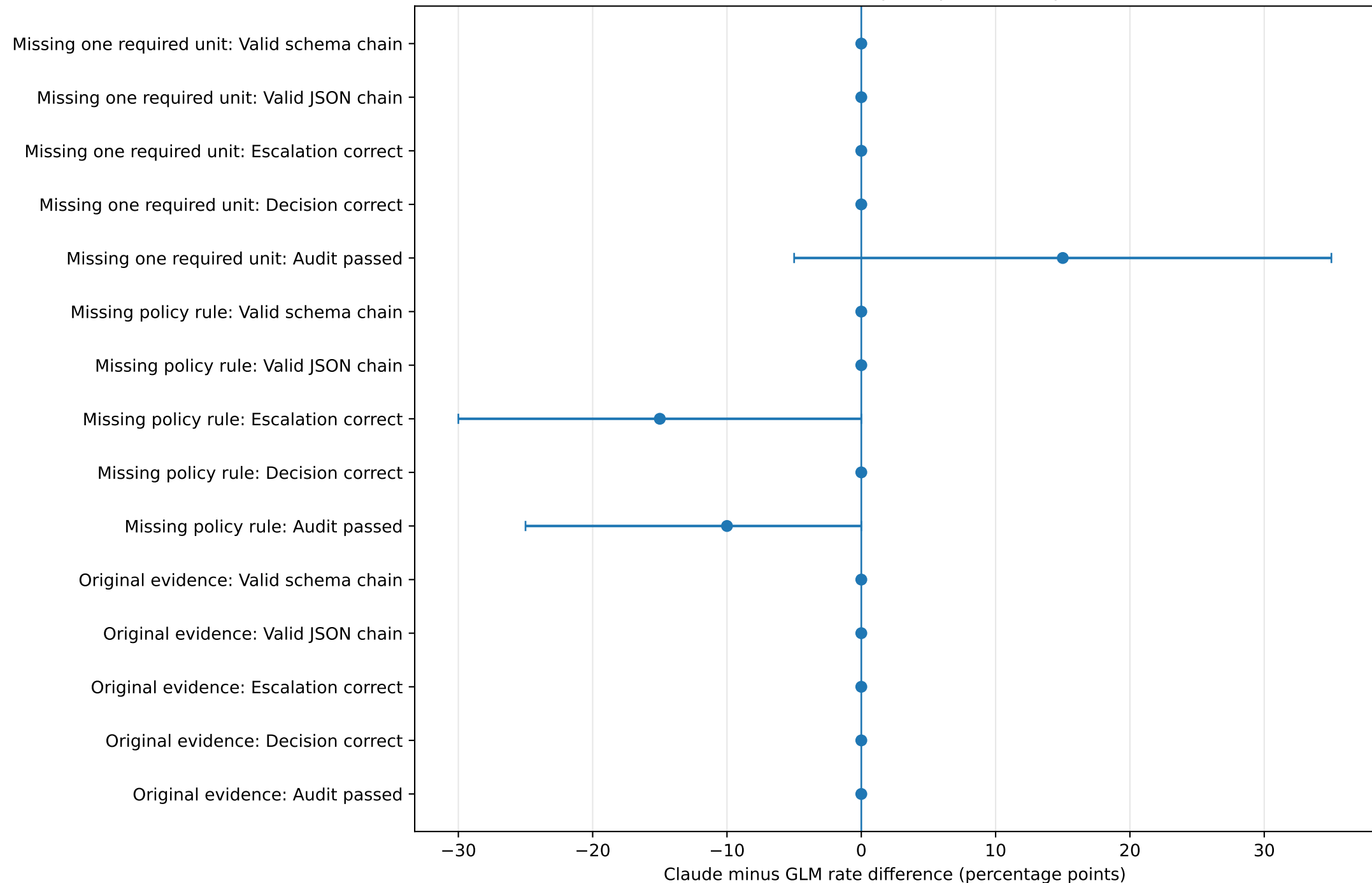
GLM vs Claude descriptive paired comparison
