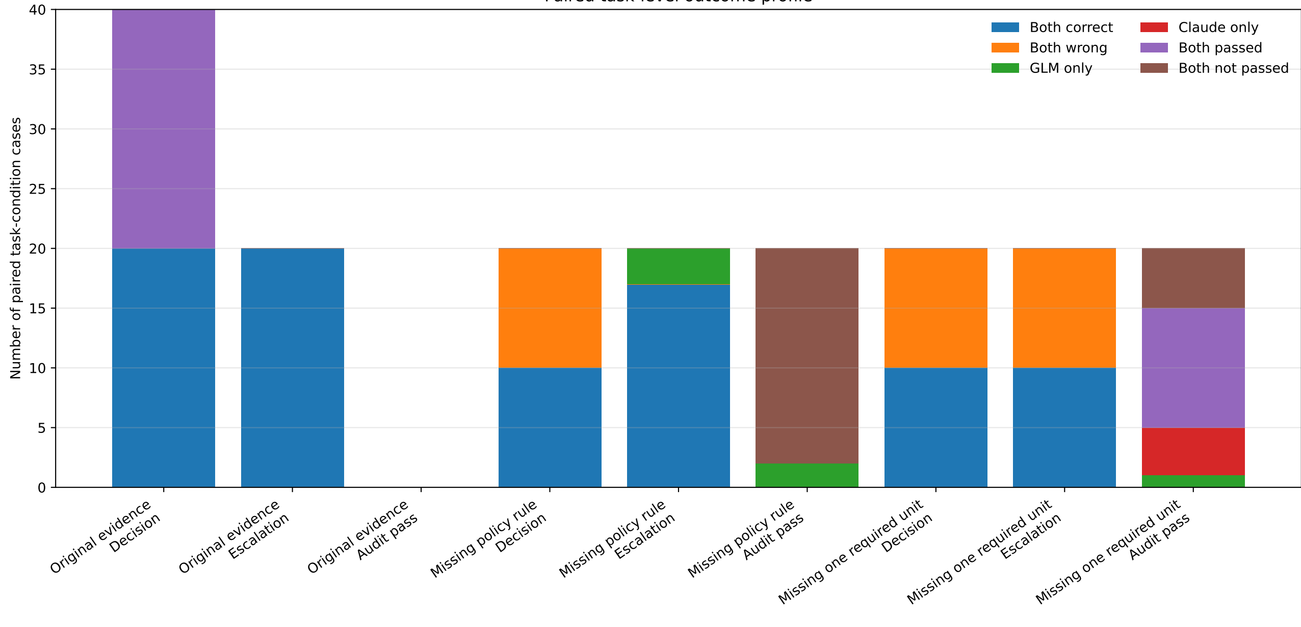
Paired task-level outcome profile
