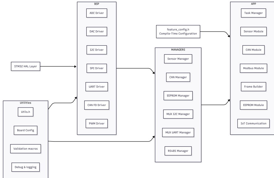
Figure 3.1: Layered software architecture of the IOBOX platform
