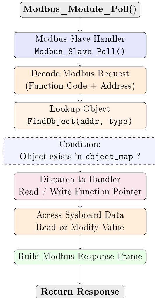
Figure 3.4: Modbus Module Polling and Object Access Flow
