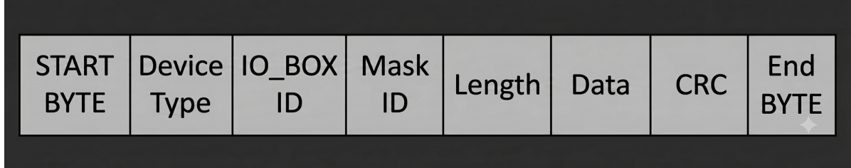
Figure 3.2: Structure of the IOBOX output frame ( IoFrame )
