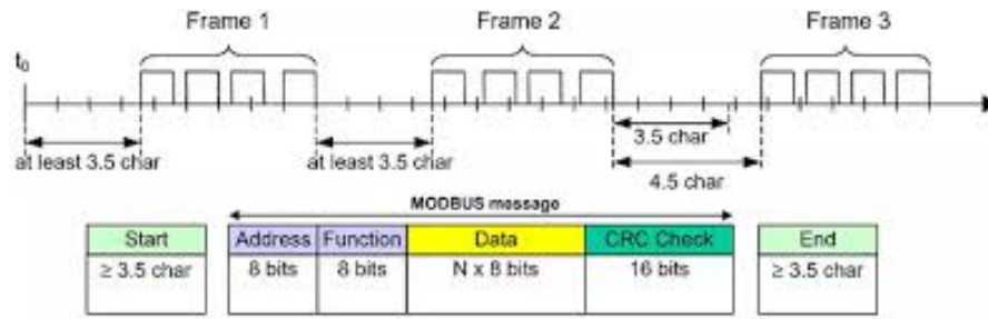
Figure 2.15: Typical Modbus RTU frame structure
