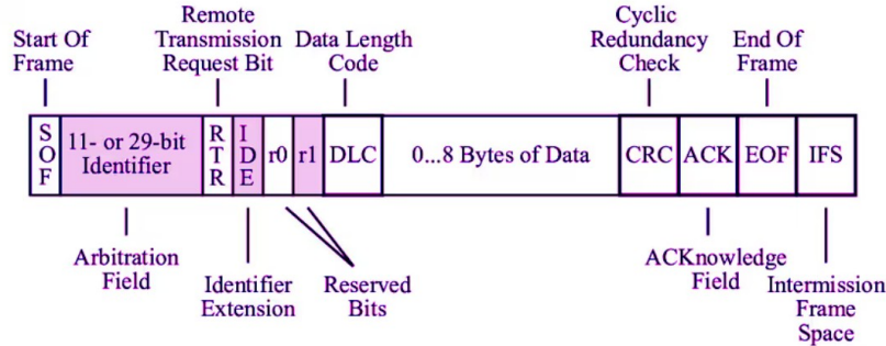
Figure 2.16: Basic CAN frame
