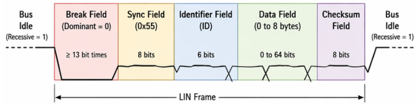
Figure 2.18: LIN frame structure
