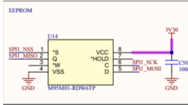
Figure 2.1: M95M01-RDW6TP EEPROM memory chip
