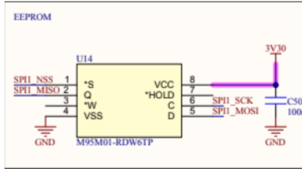
Figure 2.2: M95M01-RDW6TP EEPROM memory chip
