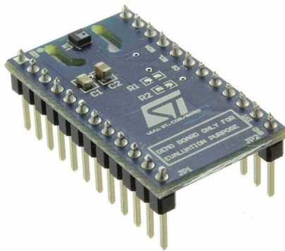
Figure 2.5: HTS221TR temperature and humidity sensor
