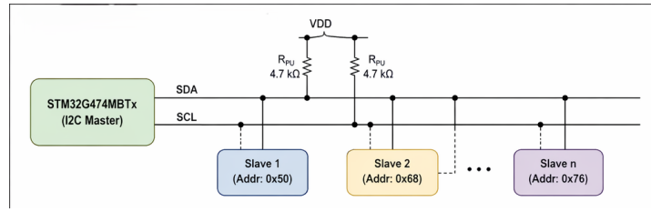
Figure 2.11: I2C communication bus architecture
