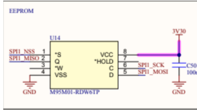
Figure 2.2: M95M01-RDW6TP EEPROM memory chip
