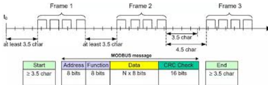
Figure 2.15: Typical Modbus RTU frame structure
