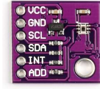
Figure 2.3: OPT3001DNPR ambient light sensor
