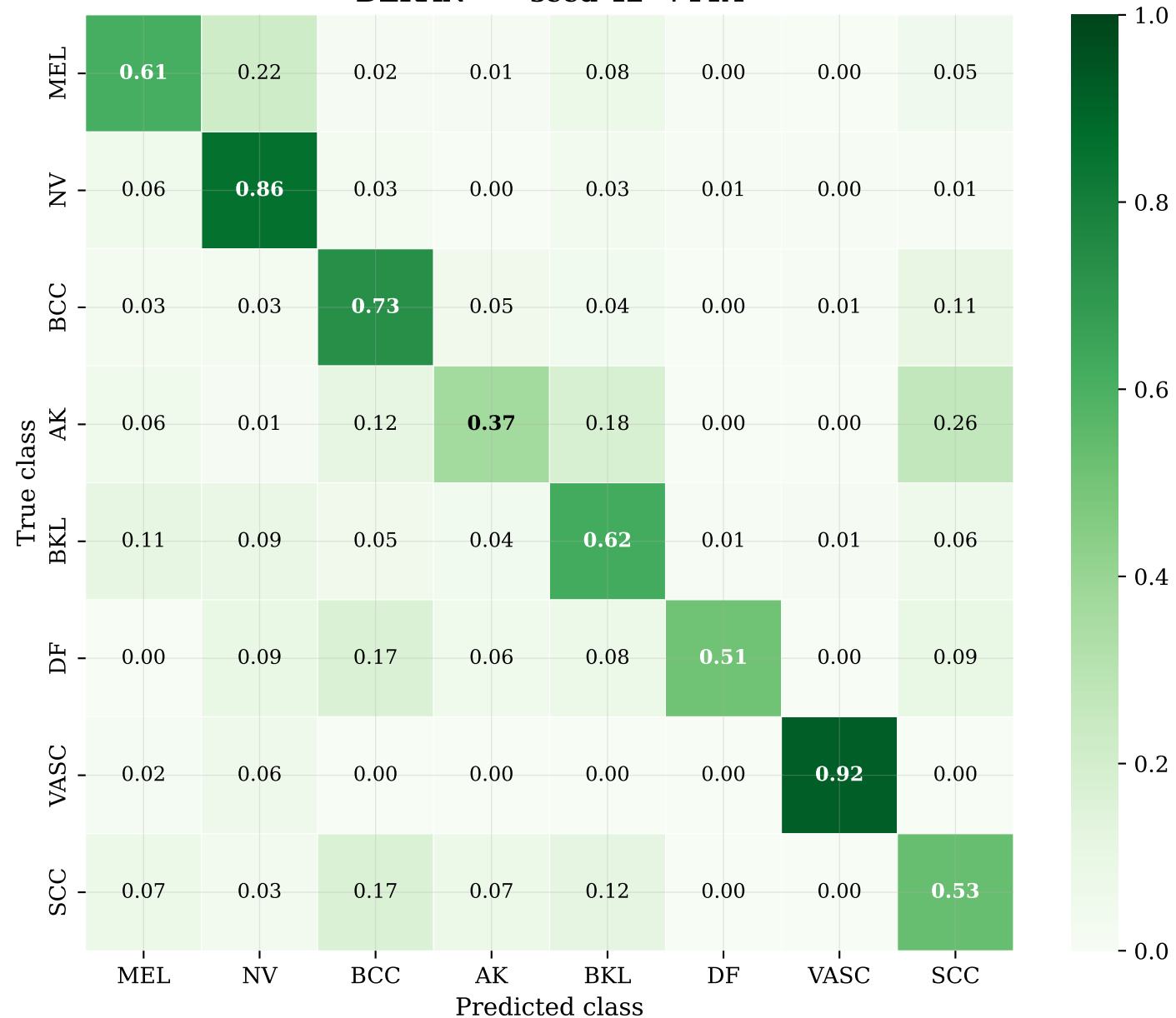
Confusion Matrix (normalised by true class)
