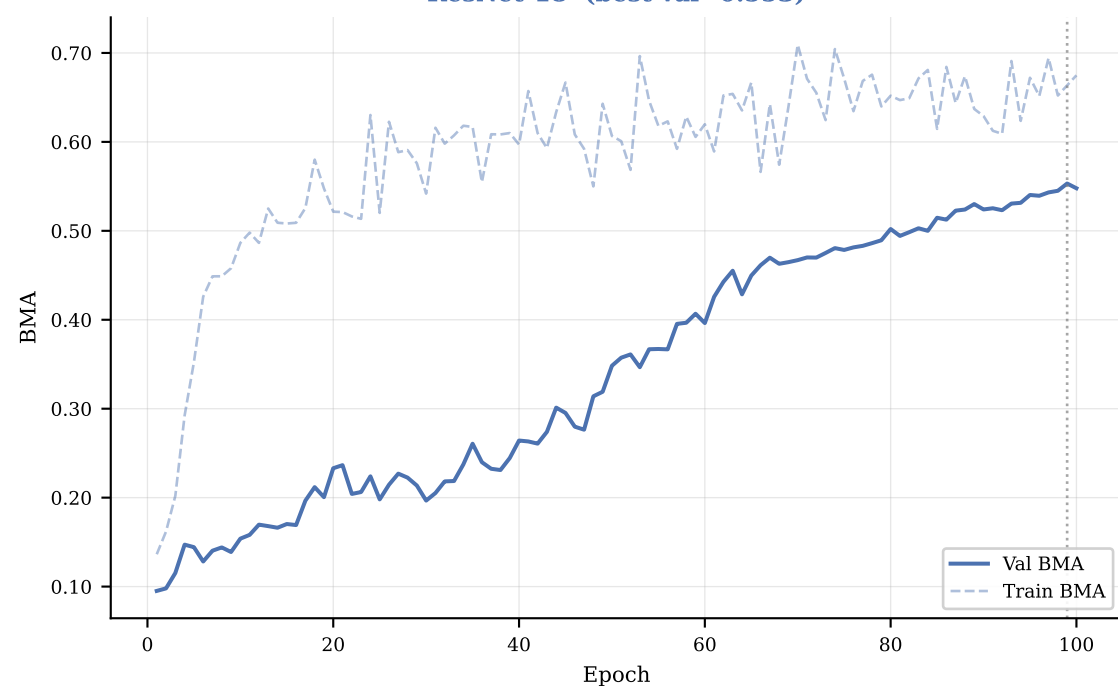
Training Curves — All Main Models (BMA vs Epoch, seed 42) Dashed = train BMA, solid = val BMA, dotted line = best val checkpoint ResNet-18 (best val=0.553) MobileNetV2 (best val=0.487)
