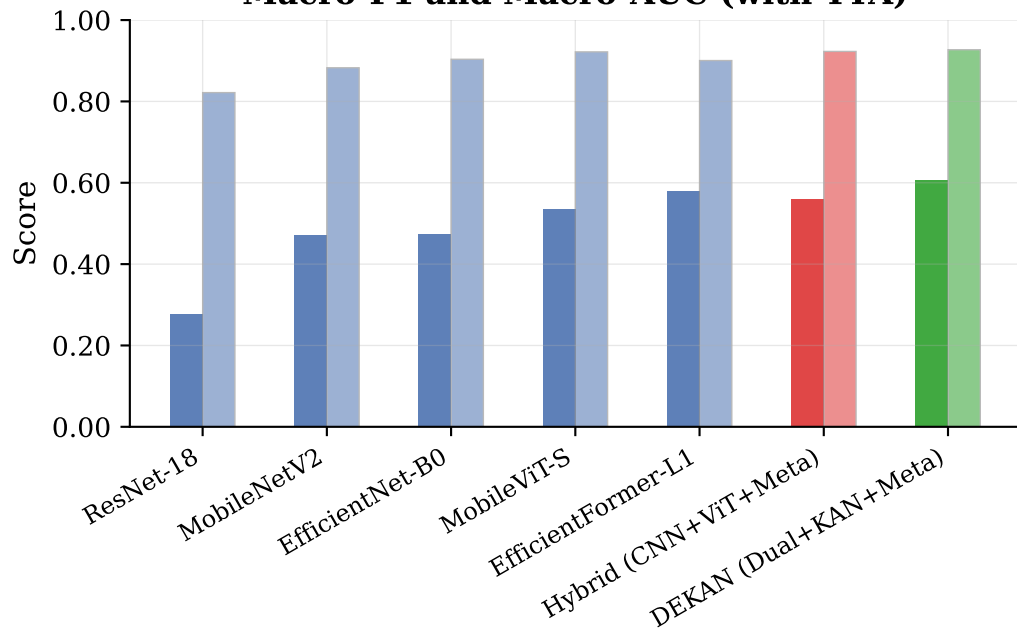
Macro-F1 and Macro-AUC (with TTA)
