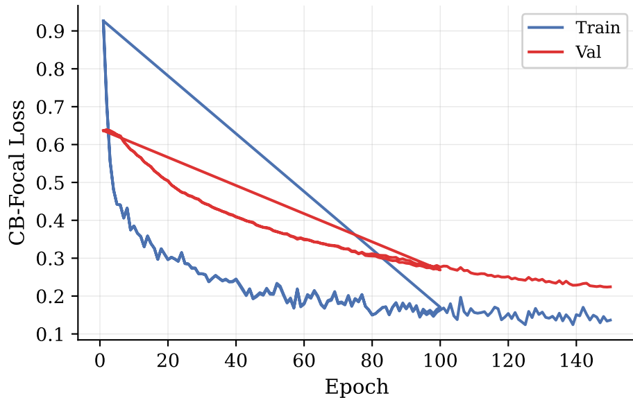
Training & Validation Loss
