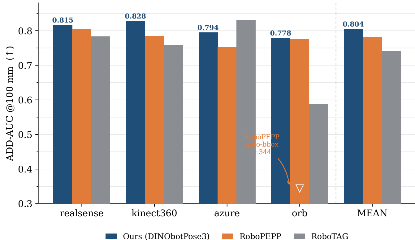
DREAM real (Franka Panda) — ADD-AUC@100mm, 1000-frame re-lock ours: predicted angles + automatic bbox vs published baselines
