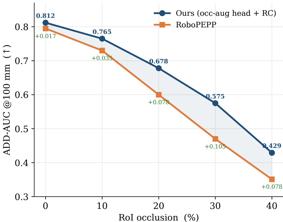
Occlusion robustness (RoboPEPP Fig. 6 protocol) ours beats at every level
