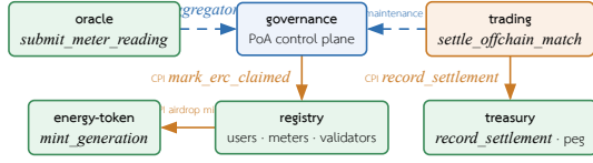
Fig. 7. Inter-program relationships among the six Anchor programs. Solid arrows are Cross-Program Invocations that write state (governance→registry on REC issue, registry→energy-token on airdrop, trading→treasury on settlement). Dashed arrows are control-plane reads with no CPI: trading reads governance for the maintenance gate and REC validity, and oracle validates an admitted-aggregator entry before accepting a reading. Governance (blue) is the policy source; trading (orange) initiates on-chain settlement.
