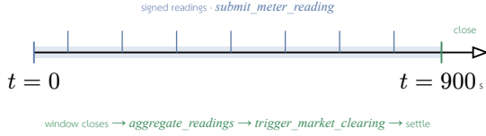
Fig. 8. Market-clearing timeline: signed meter readings ingest continuously over the 15-minute (900 s) aggregation window; at window close the oracle aggregates readings, triggers clearing, and the matched pair is settled on-chain.
