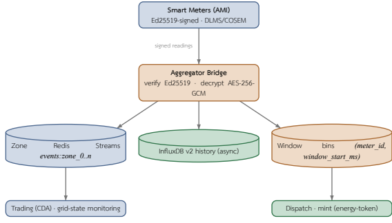
Fig. 5. Aggregator Bridge telemetry dissemination: verified readings fan out to zone-partitioned Redis Streams (real-time), an InfluxDB history sink (async, fire-and-forget), and 15-min aggregation windows keyed by (meter_id, window_start_ms) . Each sink sits above the consumer it feeds; the InfluxDB history sink is terminal.
