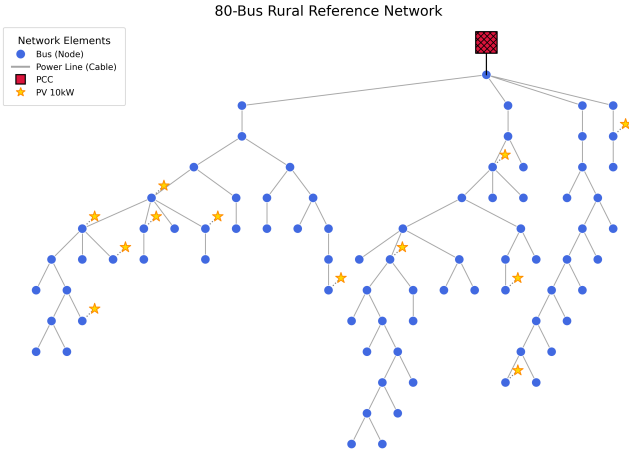
Fig. 4. Grid bus network topology used by the simulator.
