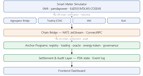
Fig. 1. Layered system architecture: off-chain verification/matching decoupled from on-chain settlement.
