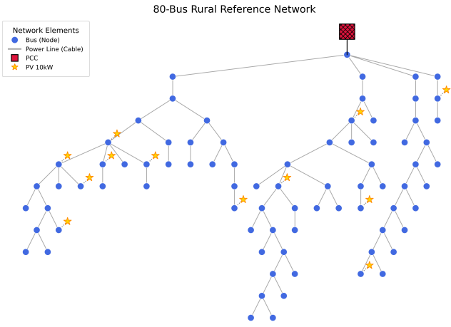
Fig. 2. Grid bus network topology used for simulator.
