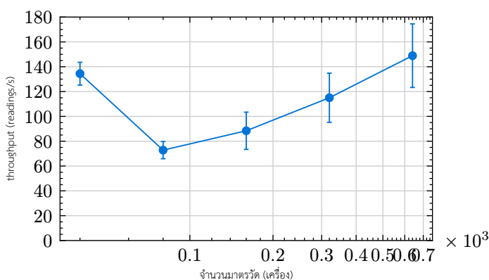
Fig. 5. Ingest throughput (mean ± sd) vs. meter-fleet size; loss stays \leq 0.03\% and no saturation knee appears within the tested range.
