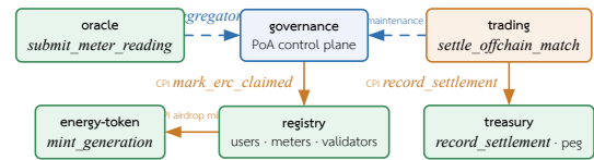
รูปที่ 6. Inter-program relationships among the six Anchor programs. Solid arrows are Cross-Program Invocations that write state (governance→registry on REC issue, registry→energy-token on airdrop, trading→treasury on settlement). Dashed arrows are control-plane reads with no CPI: trading reads governance for the maintenance gate and REC validity, and oracle validates an admitted-aggregator entry before accepting a reading. Governance (blue) is the policy source; trading (orange) initiates on-chain settlement.
