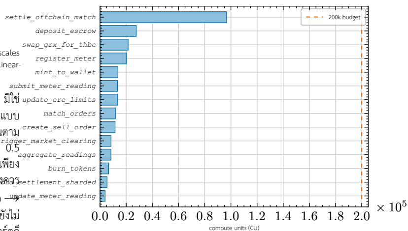
รูปที่ 11. Measured per-instruction compute-unit cost across the on-chain programs (litesvm computeUnitsConsumed , default-feature build; settle_offchain_match measured on a live validator per หัวข้อ X.E), sorted by cost. Only the signature-verifying settlement path approaches half the 200,000 CU per-instruction budget (dashed); every other instruction stays well below — the measured signature of a thin settlement layer.
