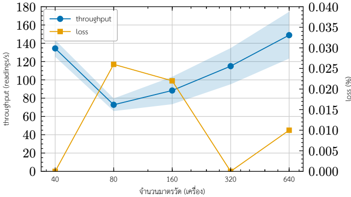
รูปที่ 9. Ingest throughput (left axis, mean ± sd) and request loss (right axis) vs. meter-fleet size; loss stays ≤ 0.03% across the tested range. Throughput is non-monotonic and single-client sender-bound — a lower bound, not a service-saturation curve.
