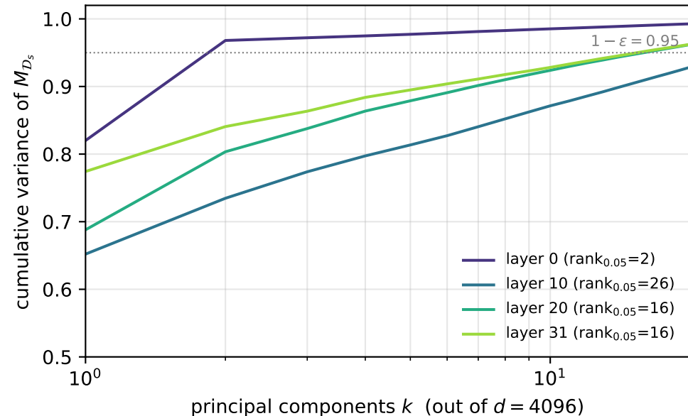
Llama-3.1-8B-Instruct
