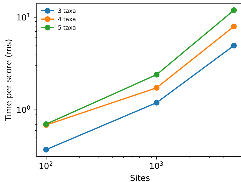
(b) Biallelic-marker likelihood
