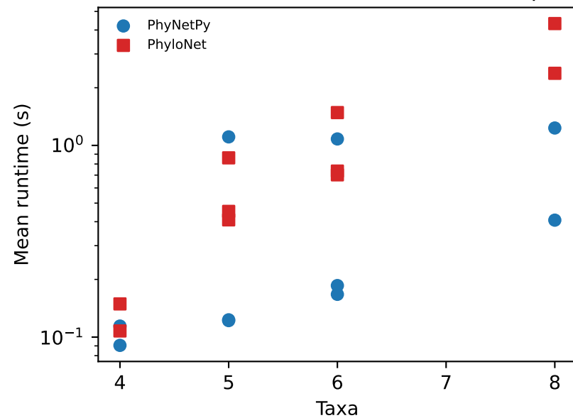
(a) Pseudo-likelihood search, same input
