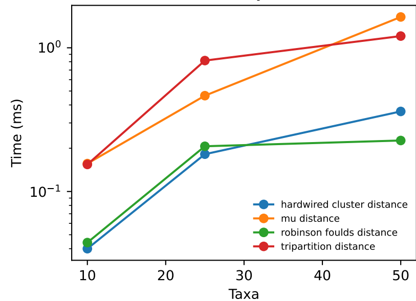
(c) Dissimilarity measures
