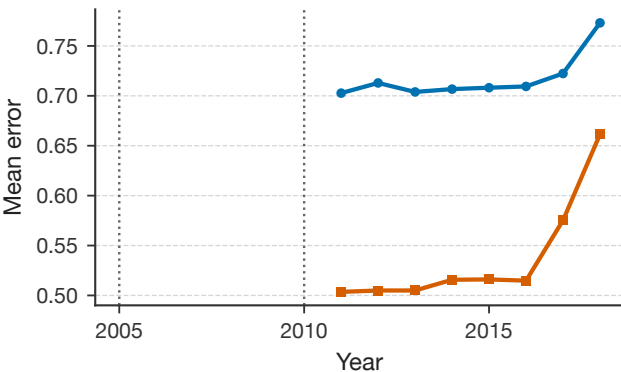
Ordinary SWD
