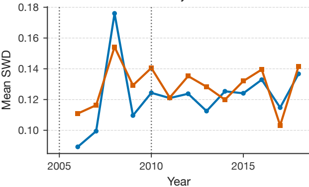
Ordinary SWD
