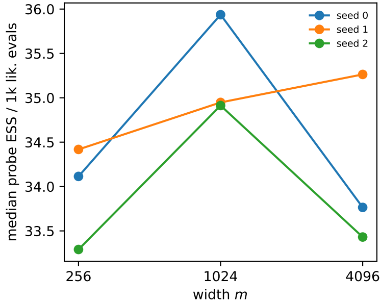
ESS per evaluation
