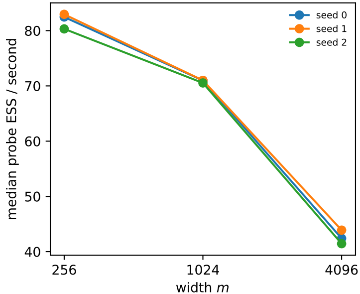
ESS per second
