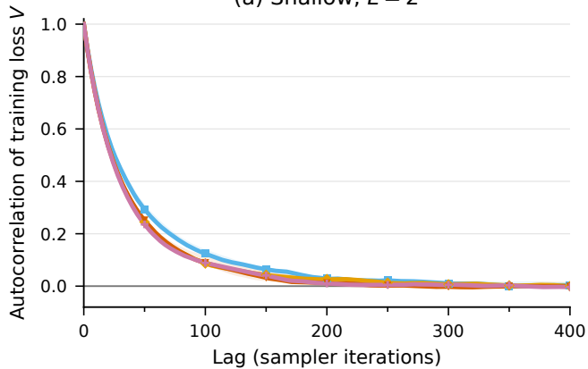
(a) Shallow, L = 2
