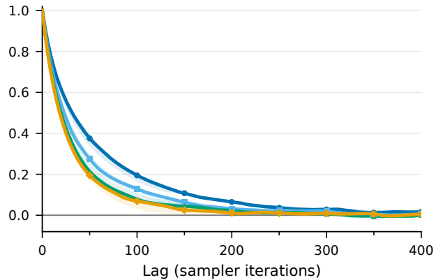
(b) Deep, L = 3
