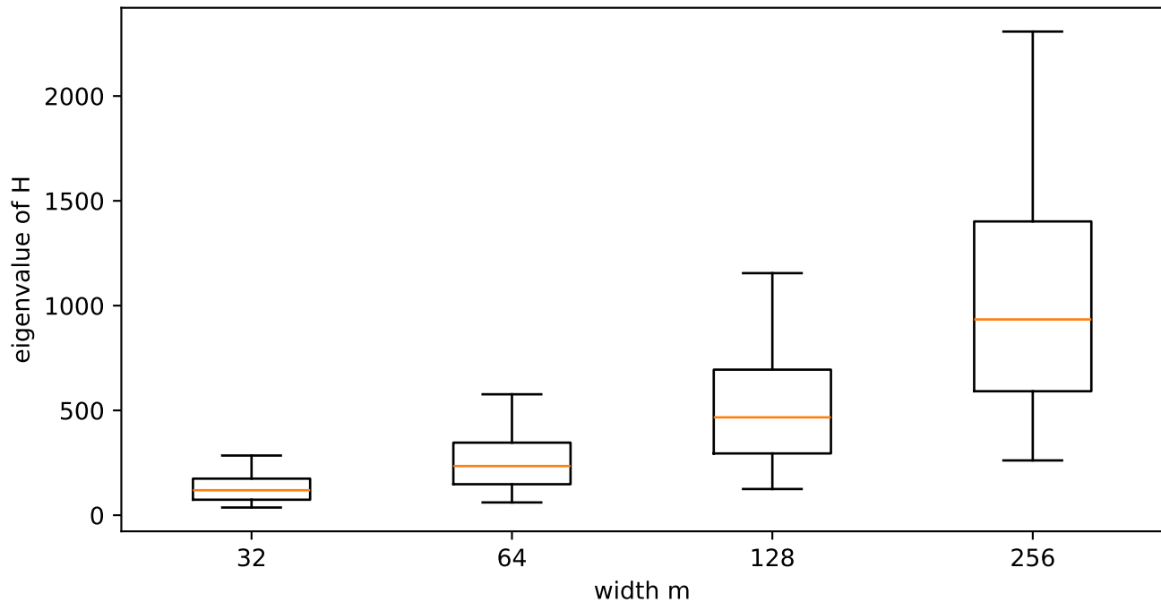
H spectrum by width (pooled seeds)
