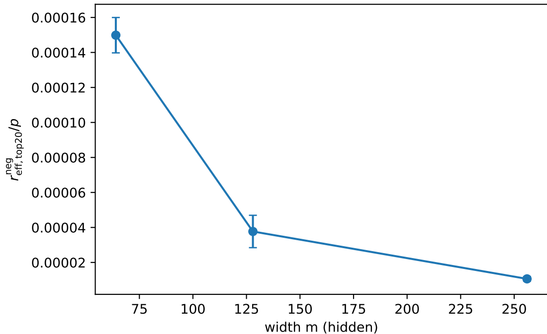
effective negative rank (top-20) / p (checkpoint=final)
