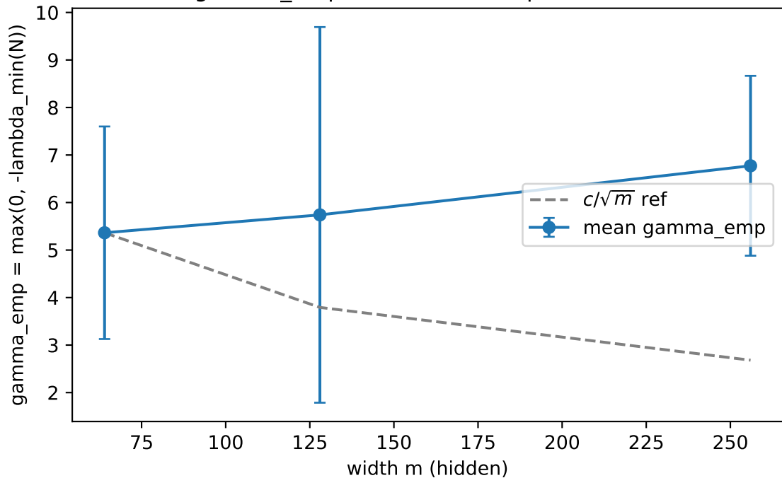
gamma_emp vs width (checkpoint=final)
