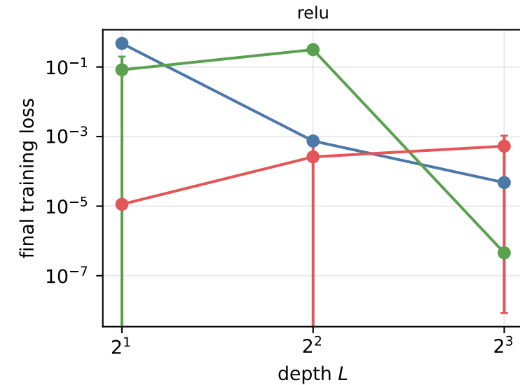
Depth sweep (MNIST-1D, width 128, 12k steps). PARTIAL: deeper cells still running.
