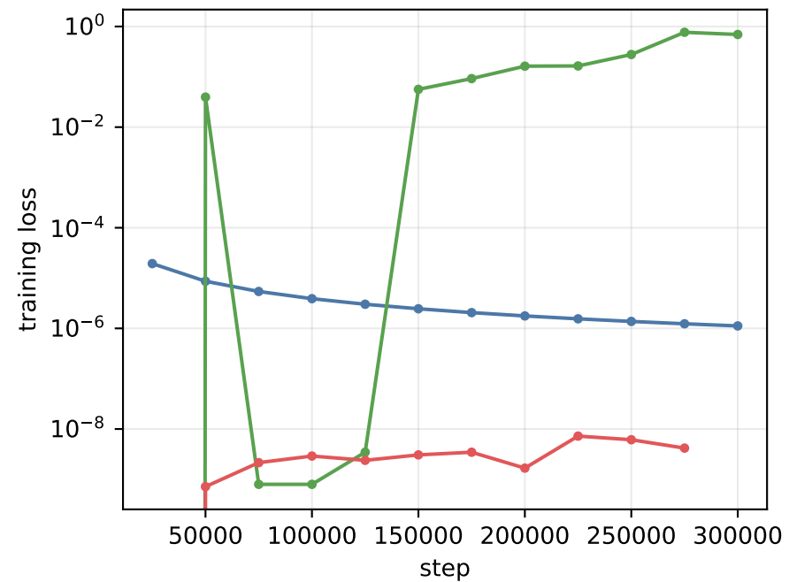
relu: extended training, every tracked statistic
