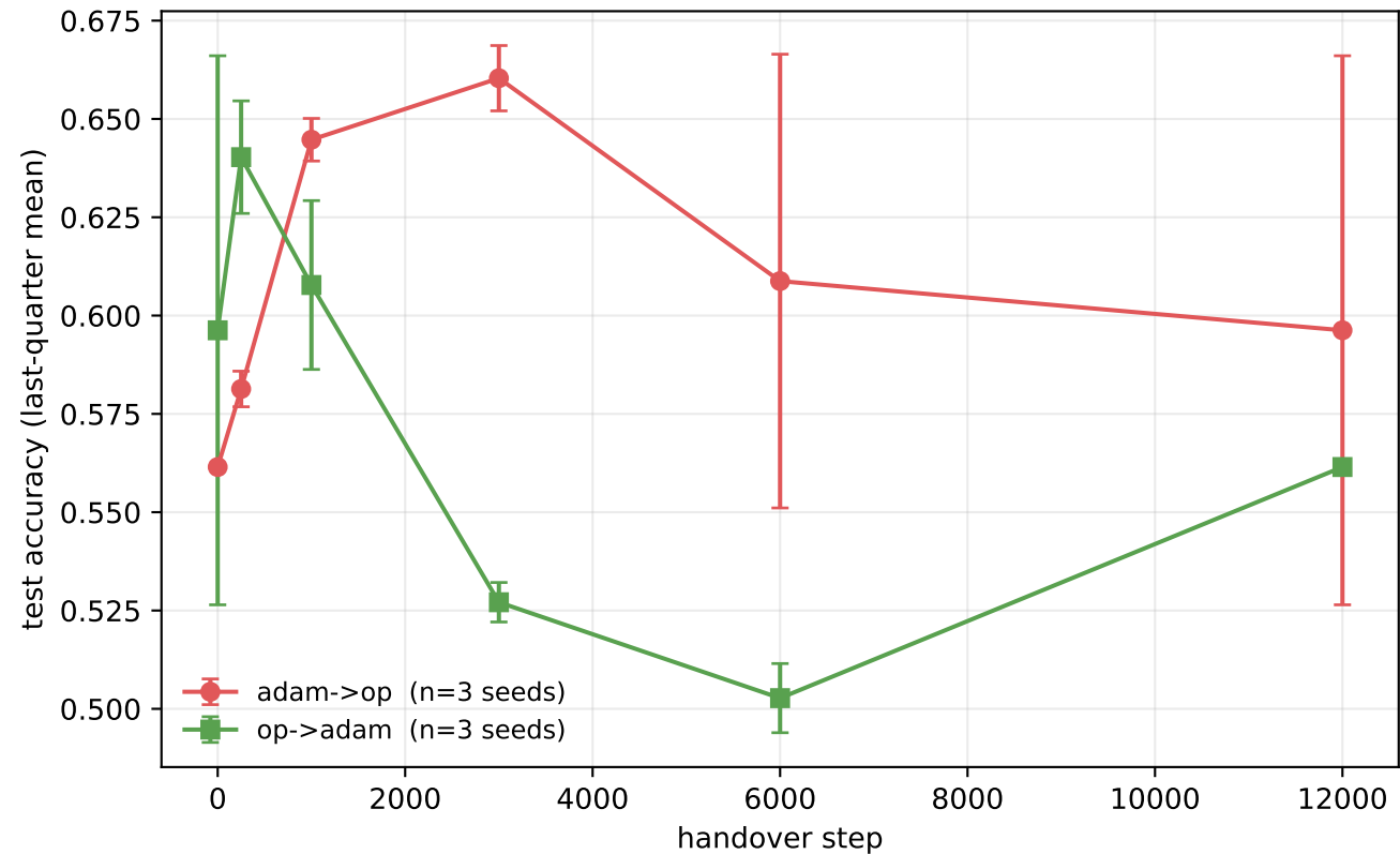
crelu: when is the advantage created?
