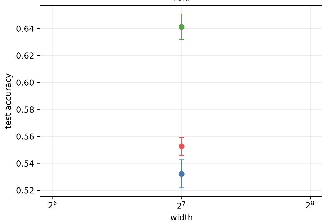
relu
