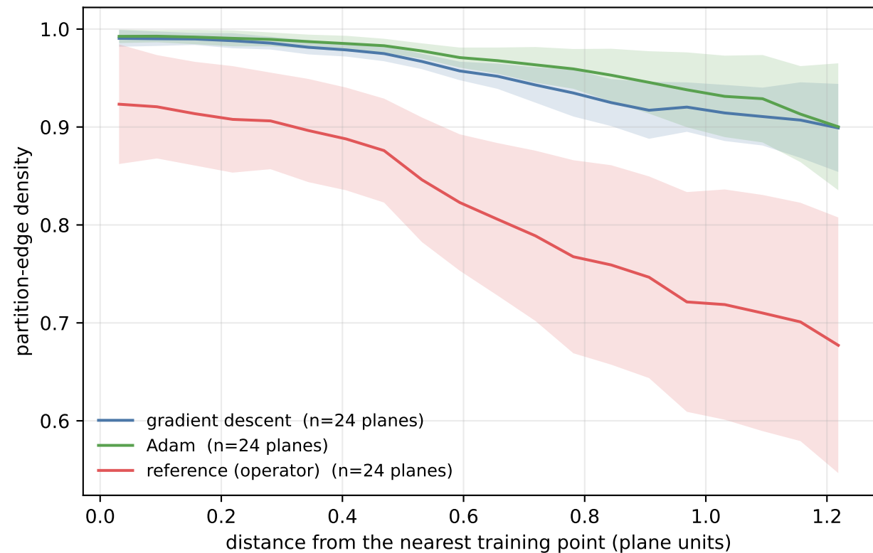
crelu: averaged over random planes and seeds (band = 1 sd)
