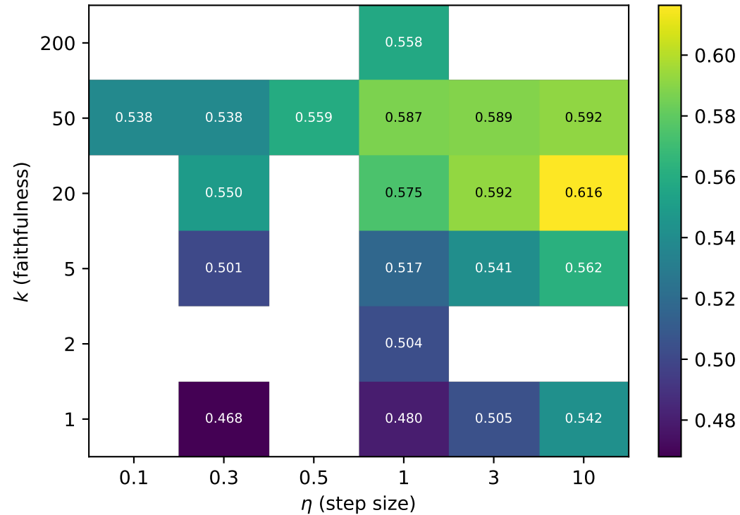
crelu: test accuracy
