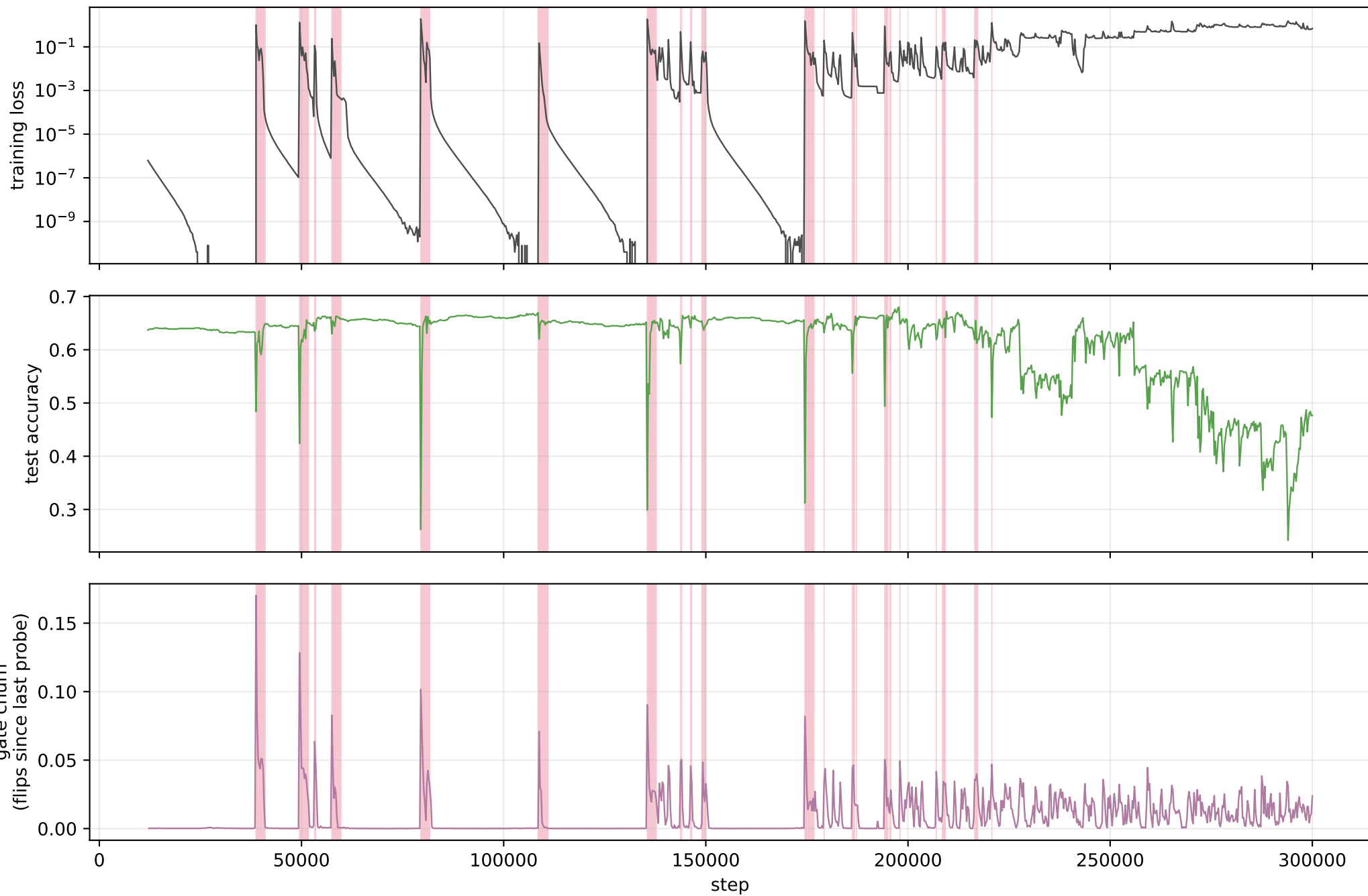
relu, Adam (hyper 0.003): loss spikes (red) against gate churn
