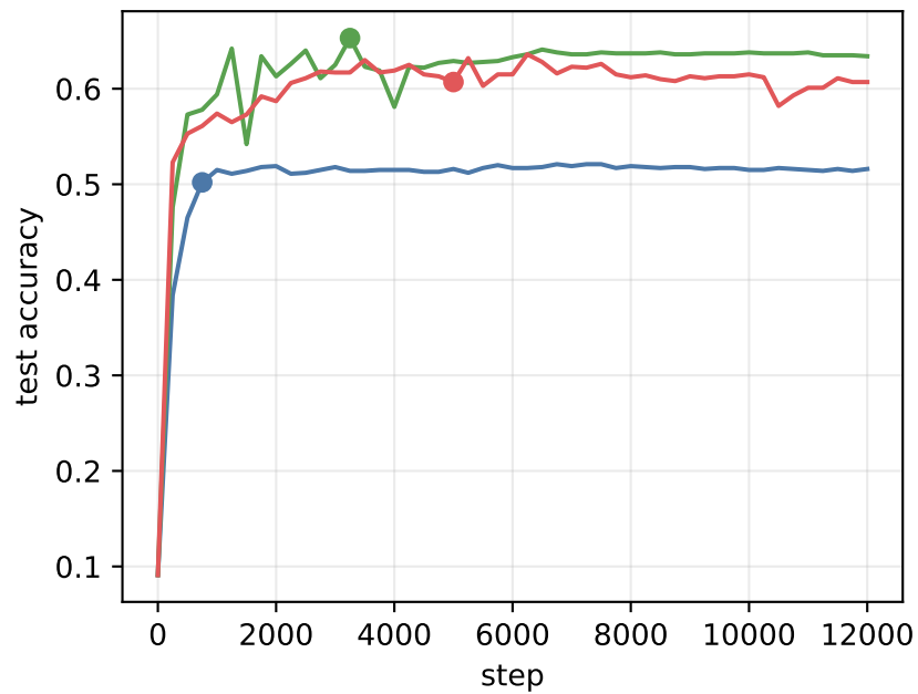
crelu, seed 0: dots mark the validation-selected point
