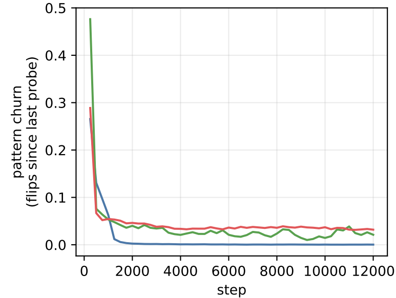
relu, seed 0
