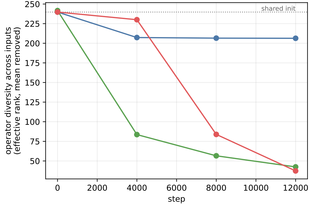
relu
