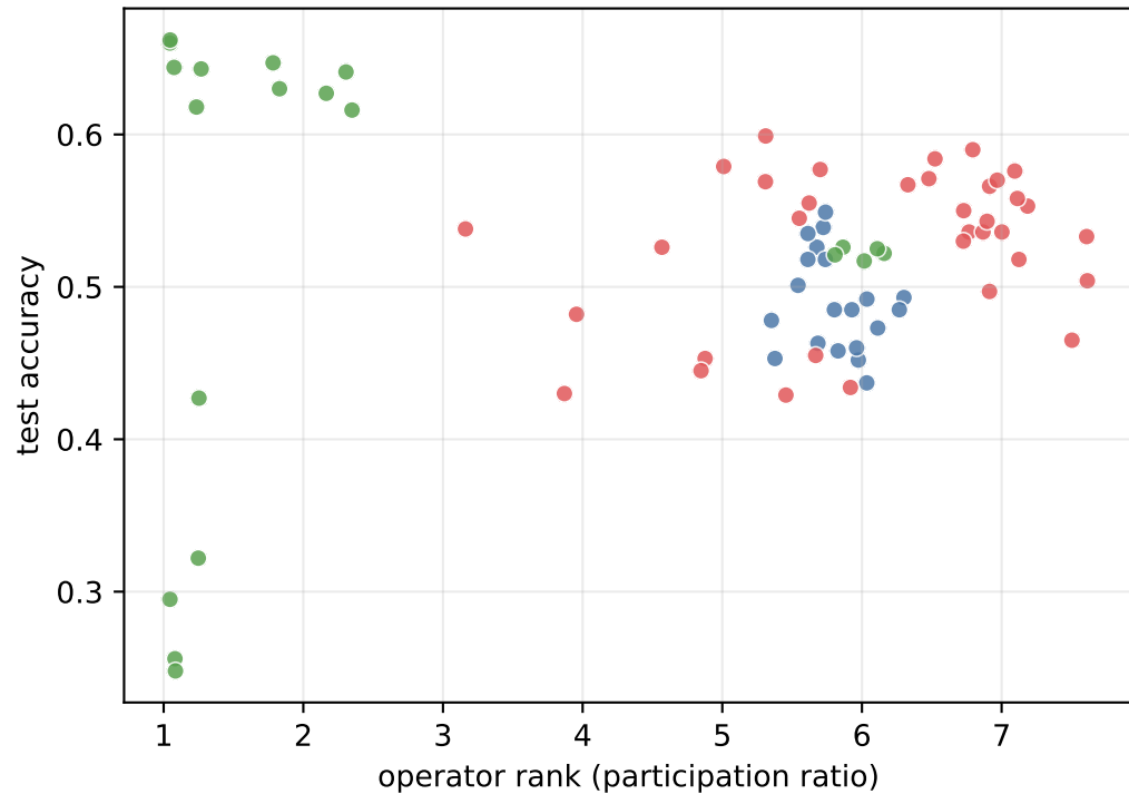
relu
