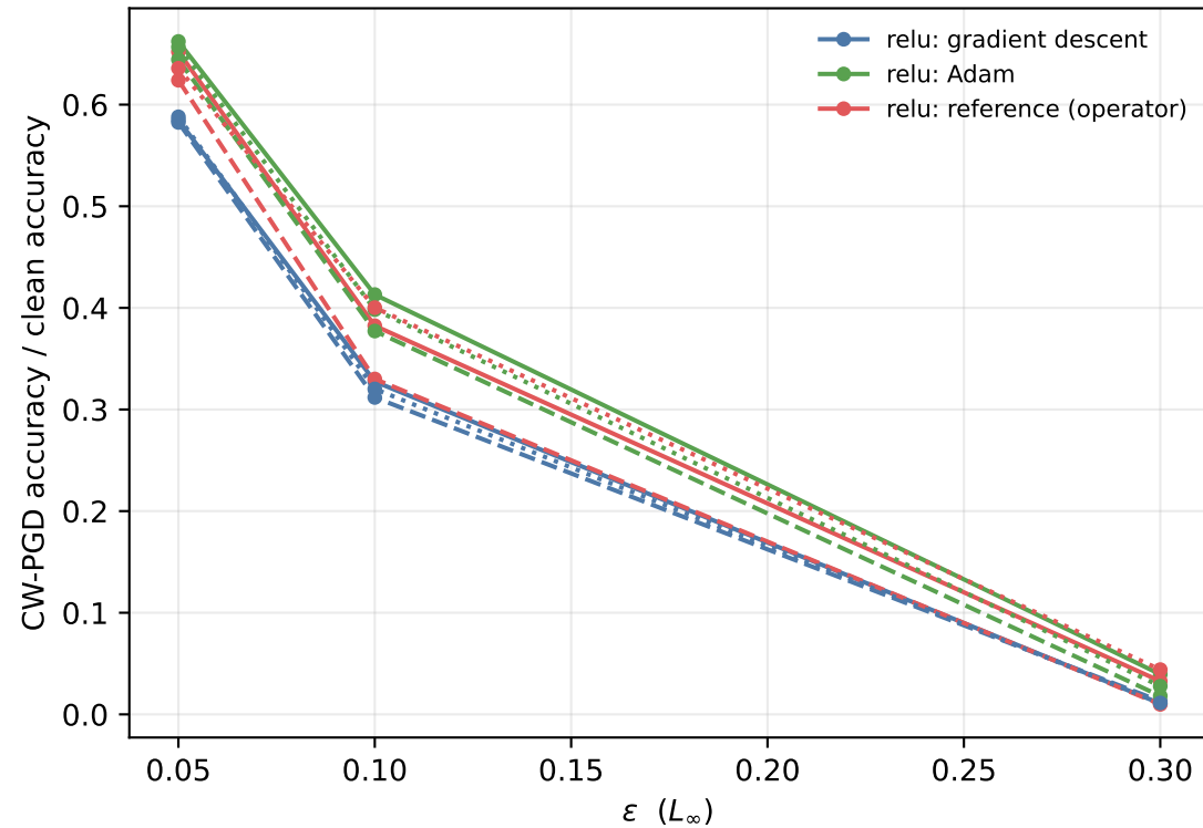
no separation survives a scale-covariant attack
