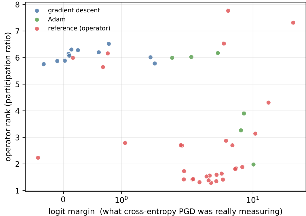
margin and rank are confounded across arms
