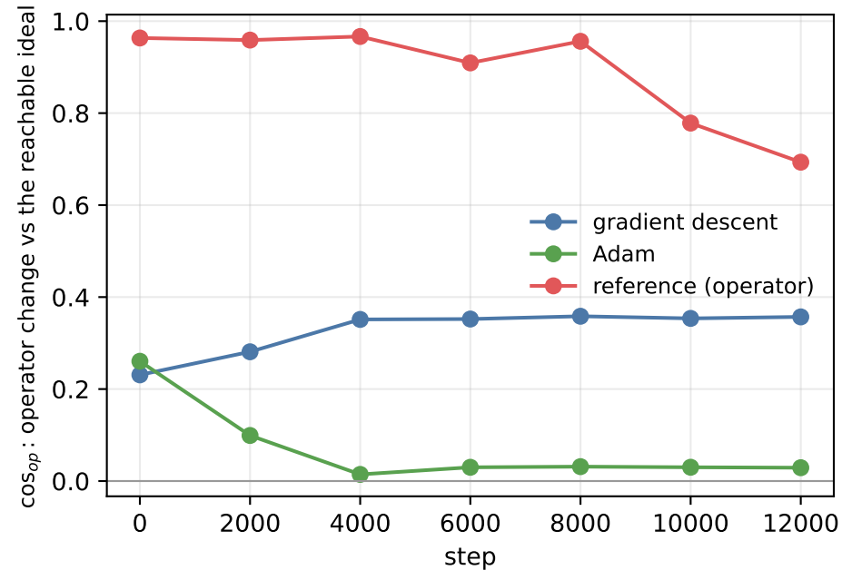
crelu, seed 0: each arm scored along its own trajectory
