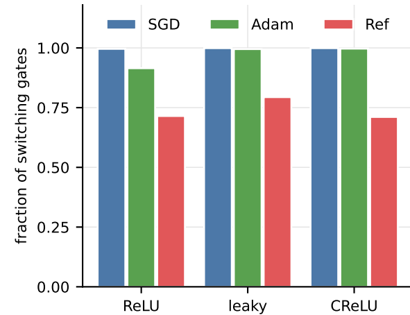
(a) input-dependent gating
