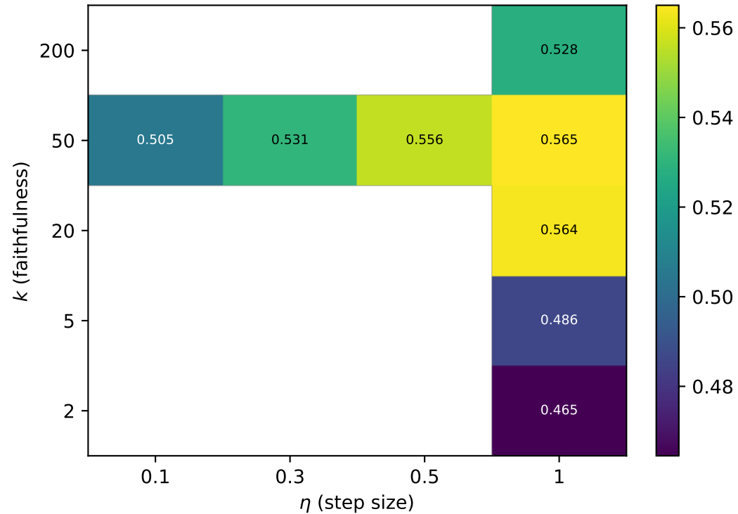
relu: test accuracy at convergence
