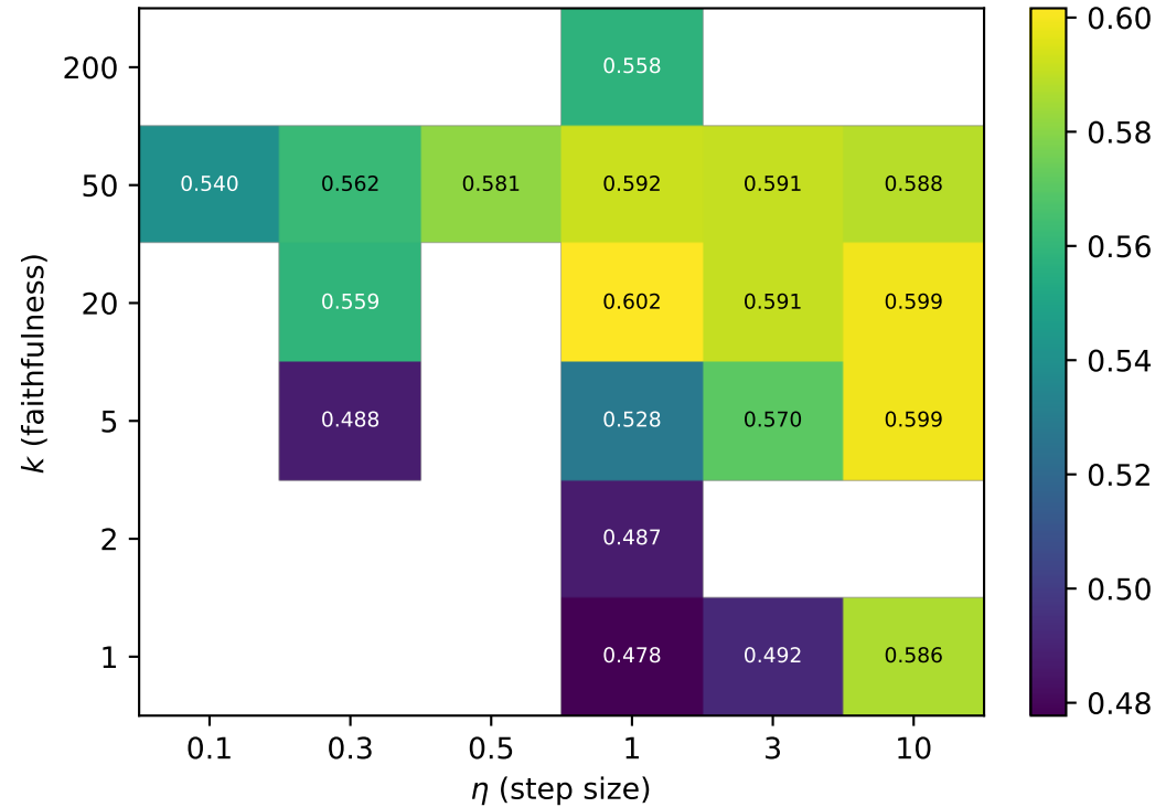
crelu: test accuracy at convergence
