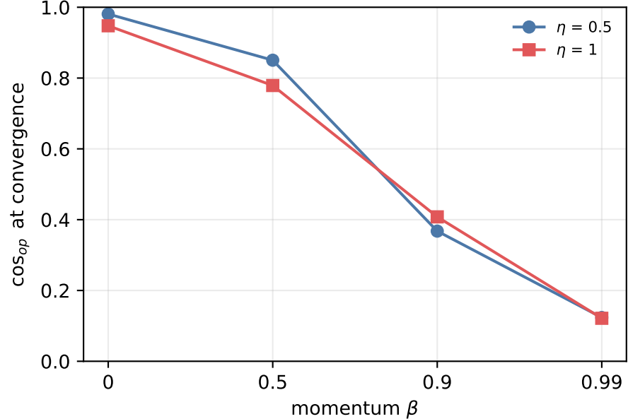
crelu: operator-space faithfulness
