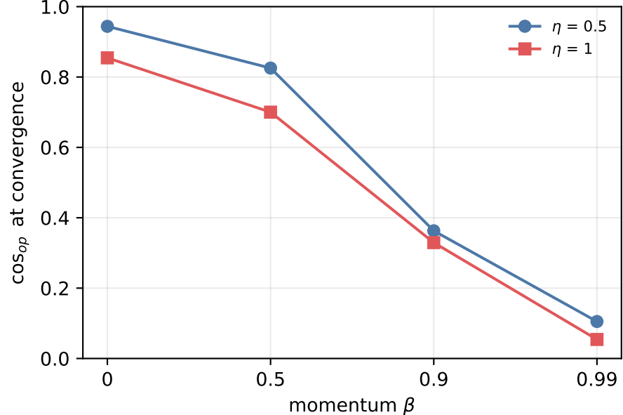
relu: operator-space faithfulness
