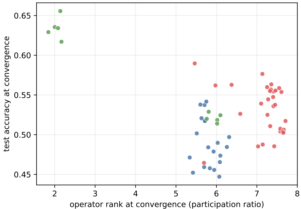
relu
