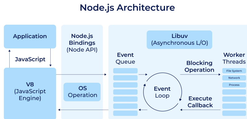
Figure 2.1: Node.js Architecture: Emphasizing Async, Event-Driven, Non-Blocking I/O
