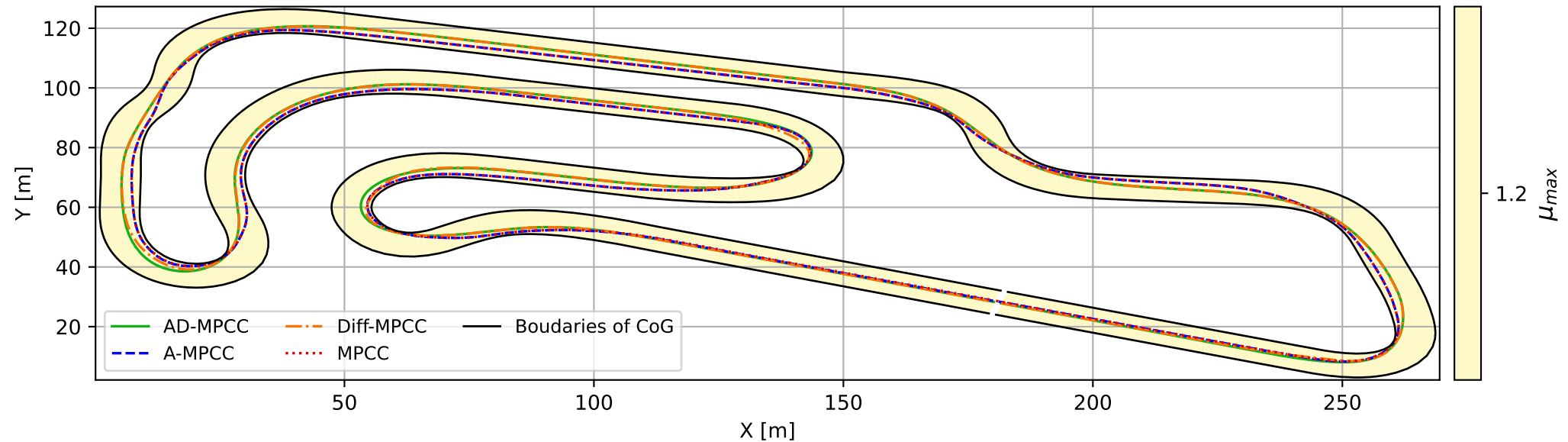
Vehicle Trajectory on Single-Surface Race Track [m]
