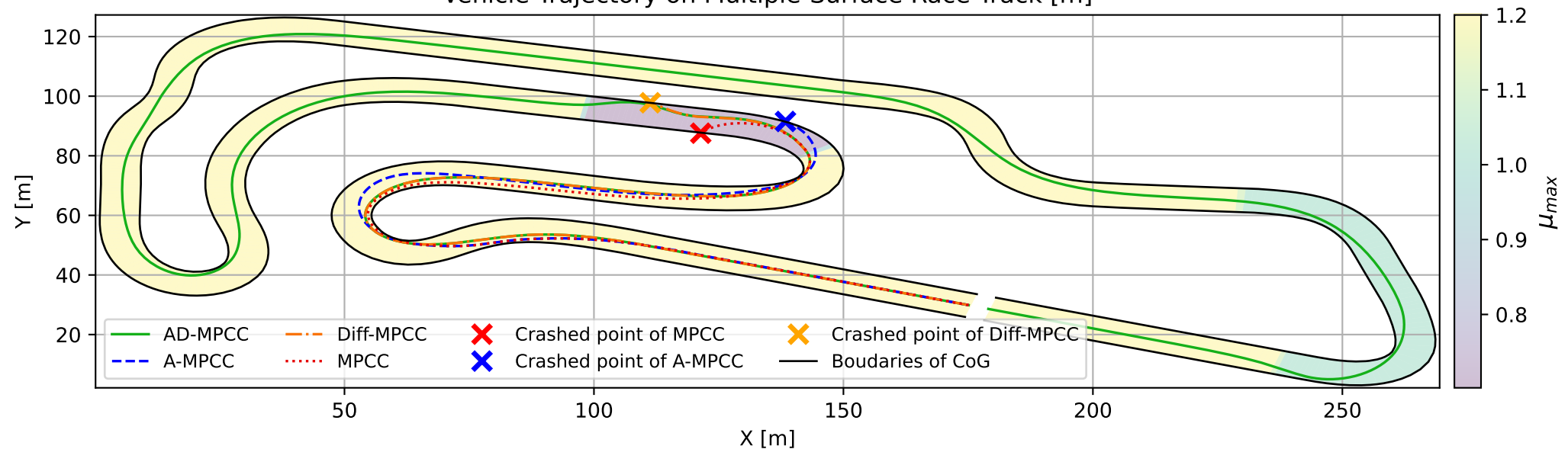
Vehicle Trajectory on Multiple-Surface Race Track [m]
