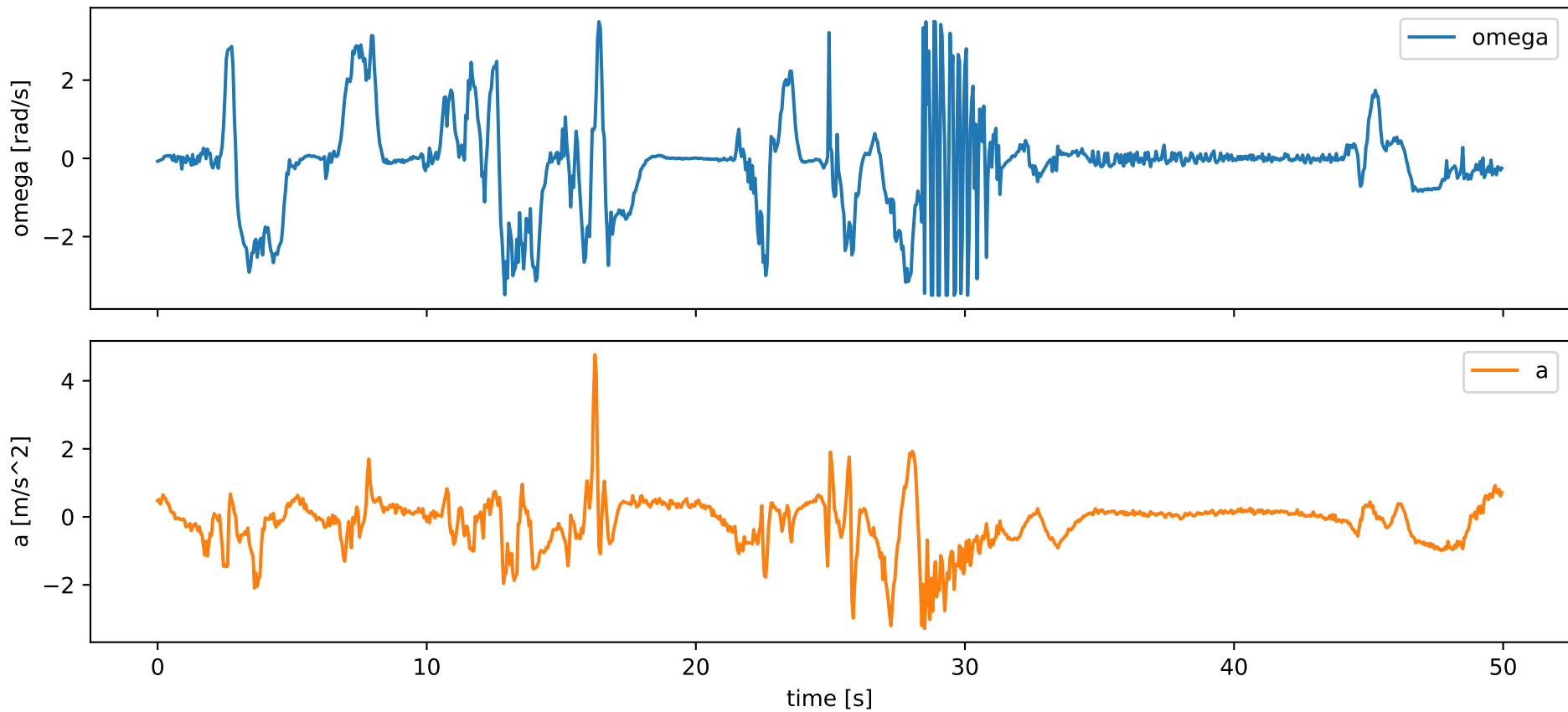
Inputs — C-MIMO DeepONet (proposed)+PANOC MPCC
